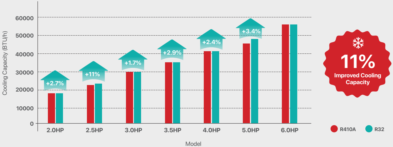
Comparison of Cooling Capacity
